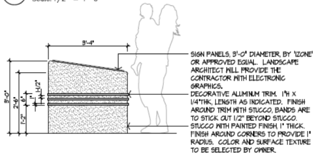
5 ELEVATION: MAP PEDESTAL Scale: 1/2" = 1'-0"
