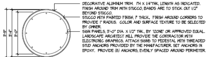
4 PLAN: MAP PEDESTAL Scale: 1/2" = 1'-0"
