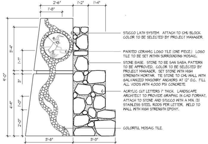
7 ELEVATION: ENTRY MONUMENT Scale: 1/2" = 1'-0"
